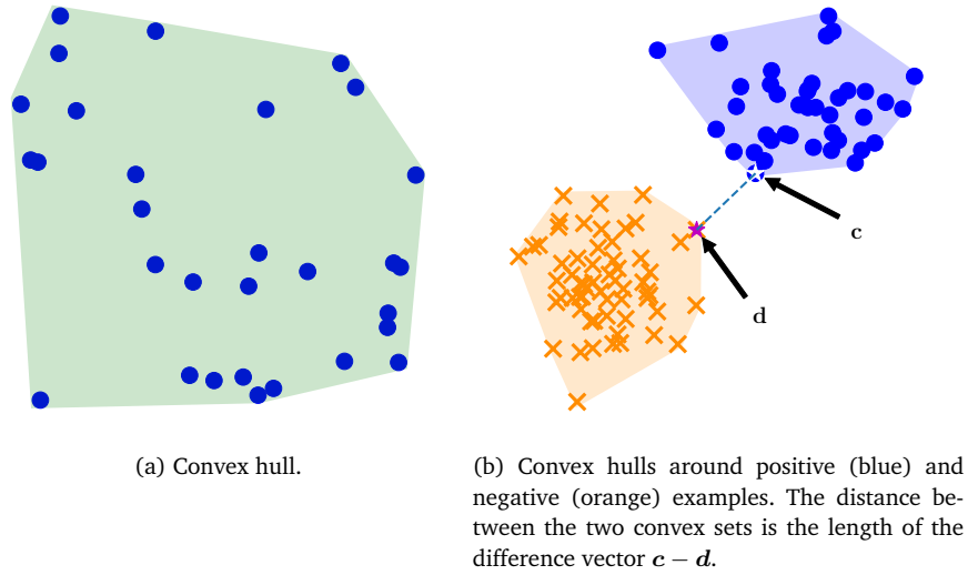
Figure 12.9 Convex hulls. (a) Convex hull of points, some of which lie within the boundary; (b) convex hulls around positive and negative examples. The distance between the two convex sets is the length of the difference vector c - d .
